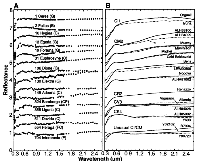
Fig. 1. (A) Telescopic reflectance spectra of the C, G, B, and F asteroids (4) and (B) laboratory reflectance spectra of carbonaceous chondrite powders (<100 or <125 \mu\text{m} ) measured at 30° incidence and 0° emergence angles. All reflectance spectra are normalized to 1.0 at a wavelength of 0.55 \mu\text{m} and shifted by 0.5 or 1.0 from each other. Class names of the asteroids are given in parentheses (1), and carbonaceous chondrite spectra are grouped according to their subgroups.
