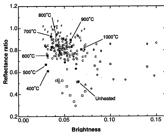
Fig. 4. A plot of the UV-visible reflectance ratio versus visible brightness of 160 C, G, B, and F asteroids and carbonaceous chondrites. The UV-visible reflectance ratio is defined as R(0.337 \mu\text{m})/R(0.55 \mu\text{m}) of the eight-color asteroid survey (8); the visible brightness is defined by the IRAS albedos for asteroids (6) and R(0.55 \mu\text{m}) for meteorites, where R(\lambda) indicates reflectance at wavelength \lambda . Class names (C, G, B, and F) are used for the asteroid points; open circles, C1; open squares, CM2; open triangles, CR2; open diamonds, CV3; inverted open triangles, CK4; closed circles, unusual CI-CM chondrites; closed squares, Murchison.
