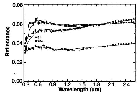
Fig. 2. Close counterparts found between the C asteroids and carbonaceous chondrites in Fig. 1. Asteroid spectra are scaled for the best fits with meteorite spectra: (top trace) 1 Ceres (G) and Y86720; (middle trace) 31 Euphrosyne (C) and B7904; and (bottom trace) 704 Interamnia (F) and Y82162. The IRAS albedos (6) of the asteroids are all scaled by 0.65 and plotted as filled circles for comparison. Vertical lines represent the standard deviation.
