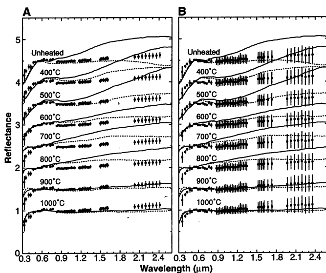
Fig. 3. Reflectance spectra of heated Murchison powders (solid trace, <63 μm; dotted trace, 63 to 125 μm) and the average reflectance spectra of (A) the five C asteroids and (B) the five G asteroids in Fig. 1. All reflectance spectra are normalized to 1.0 at a wavelength of 0.55 μm and shifted by 0.5 from each other. The standard deviations of reflectances of five asteroids are shown by vertical bars for the average C and G asteroid spectra.
