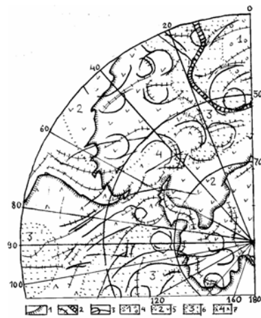
1- lines of lands, 2 –arcs and oceanic ridges, 3- lunar arcs, 4 - 6 earthen basalt fields of different ages.
