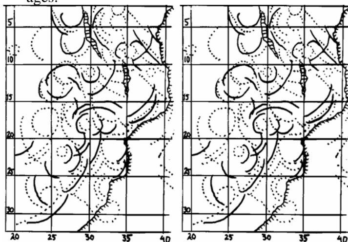
Earthen (lines ) and lunar (points) arcs,
